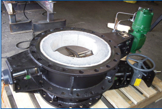
SRU Steam Jacketed Acid Gas Control BFV British Petroleum WY USA
